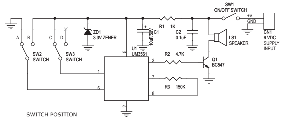
SWITCH POSITION
